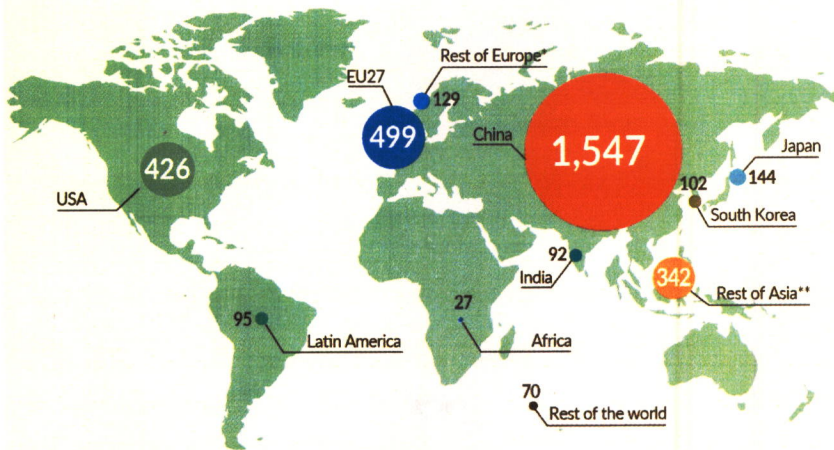
World chemical sales (2020, €3,471 billion)
